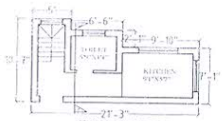
GROUND FLOOR
